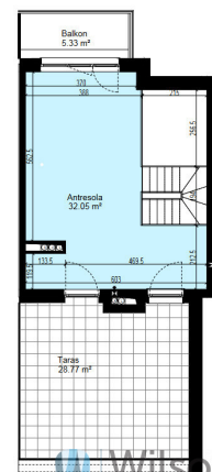
PLAN ANTRESOLI
